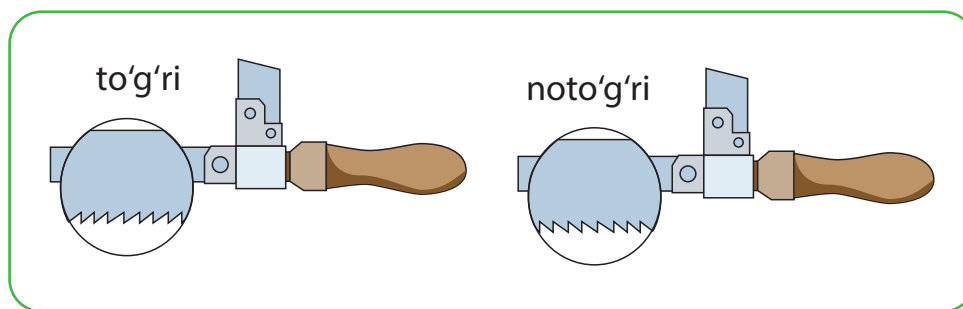
59-rasm. Polotno tishlarining o'rnatilishi
