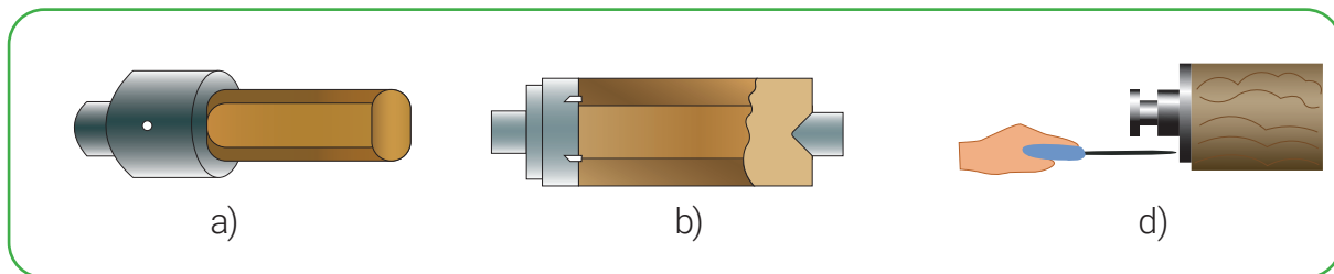
25-rasm. Tokarlik stanogida zagotovkalarni o'rnatish usullari: a) patronga o'rnatish; b) planshaybaga o'rnatish; d) trezubesga o'rnatish.
