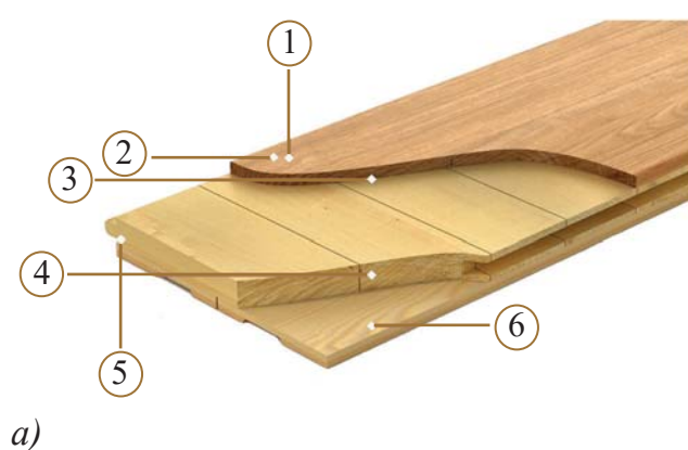
a – yog'och asosli: 1 – himoya (lok) qatlami, 2 – yuqori qatlam (faner); 3 – yelim; 4 – o'rta qatlam (taxta); 5 – ulanish qismi; 6 – pastki qatlam.
