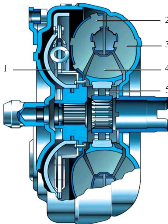
4-rasm. Gidrotransformator:
