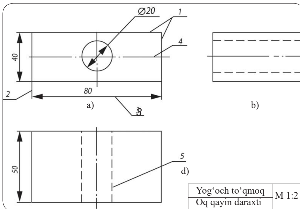
37-rasm. Buyumning eskizi.
