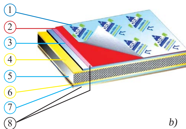
b – aluminiy asosli: 1 – himoya plyonkasi, 2 – emal; 3, 7 – aluminiy qatlami; 4, 6 – yopishqoq qatlam; 5 – plastik qatlam; 8 – himoya qatlamlari.
