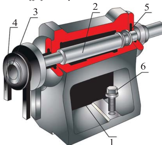
32-rasm. Oldingi babkaning tuzilishi: 1 – korpus; 2 – shpindel; 3 – ikki pog'onali shkviv; 4 – ponasimon tasma; 5 – sharchali podshipnik; 6 – qotirgich bolt.
